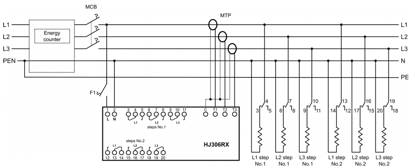
Picture 3: Connection of HJ306RX instrument
