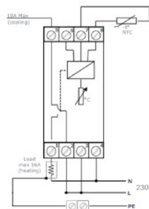
Connection scheme
